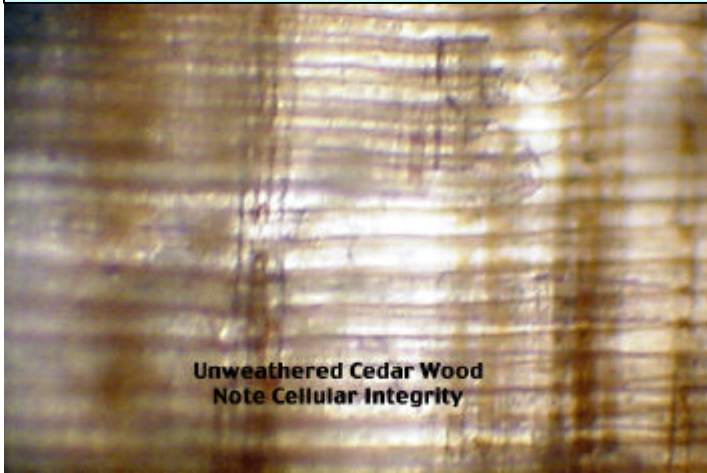
Virgin Cedar: Untreated and Unweathered
