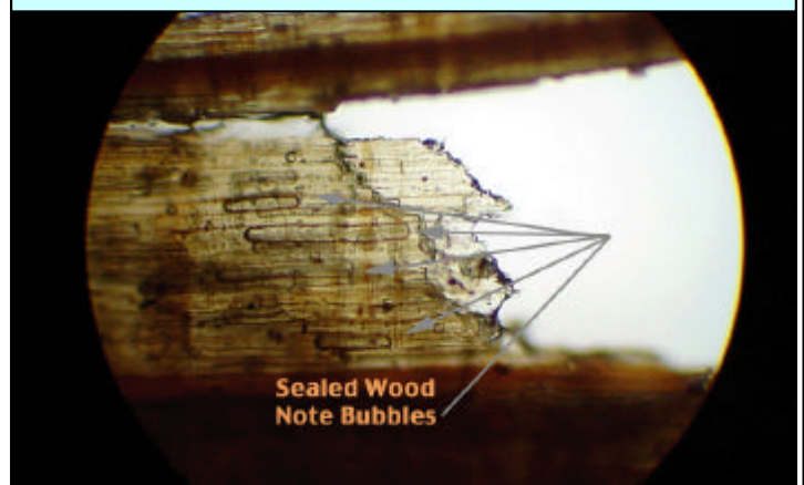
Sokol Treated Cedar Roof Shingles; Field Aged: 4 years
